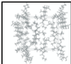
Fig. 2. The packing of the title compound, viewed along the a axis. Dashed lines indicate hydrogen bonds.
